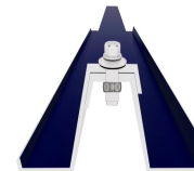
Plate assembly
